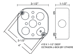
4" OCTAGONAL JUNCTION BOX DETAIL
