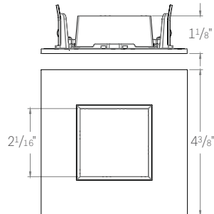
ED3-SFST SQUARE STANDARD TRIM
