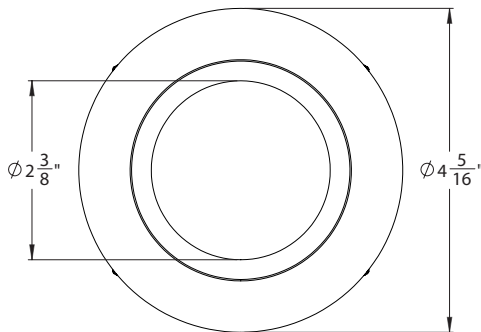
DLT3- RFST ROUND FIXED STANDARD TRIM
