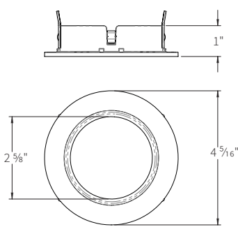
ED3-RAWR ROUND ADJUSTABLE WET LOCATION REGRESSED
