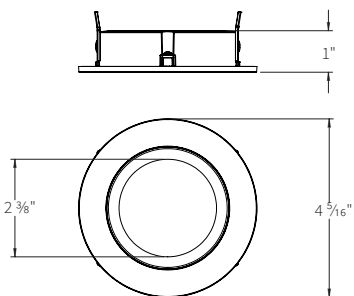
ED3-RFDF ROUND FIXED DEAD FRONT
