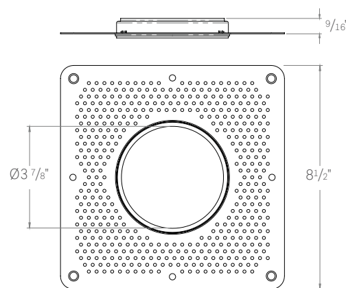
ED3-R-RMTL ROUND TRIMLESS MUDPLATE
