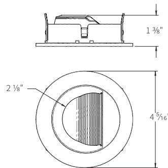
ED3-RFWW2 ROUND FIXED WALL WASH
