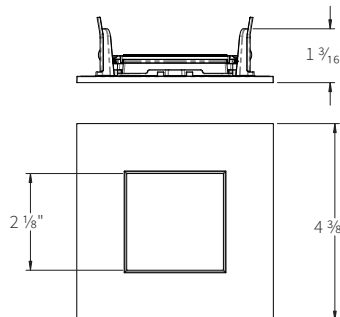
ED3-SAWR SQUARE ADJUSTABLE WET LOCATION REGRESSED
