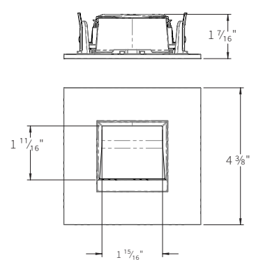
ED3-SFWW2 SQUARE FIXED WALL WASH
