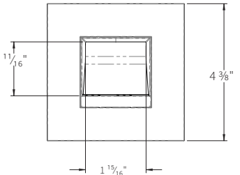
ED3-SFWW2 SQUARE FIXED WALL WASH
