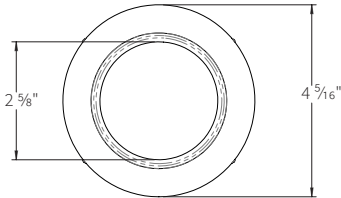
ED3-RAWR ROUND ADJUSTABLE WET LOCATION REGRESSED
