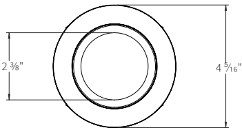
ED3-RFDF ROUND FIXED DEAD FRONT
